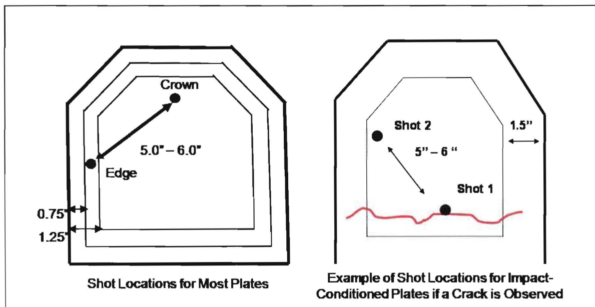
Measurements represented are for the Enhanced Small Arms Protective Insert. For the X-Small Arms Protective Insert, edge shots are between 1.0" and 1.5" from the edge.
